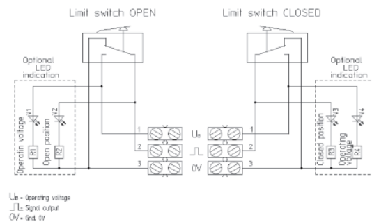
Connection diagram
